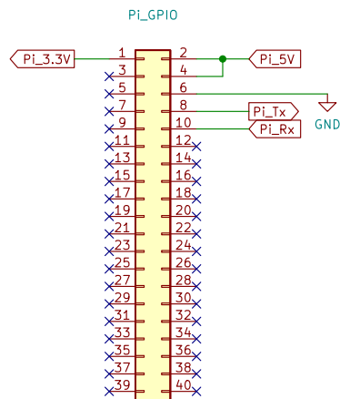
Raspberry Pi
