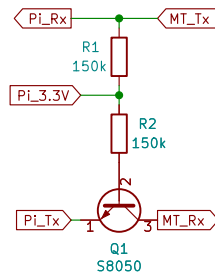
Level Shifter
